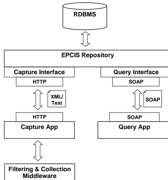
Figure 5. Accada EPCIS module featuring an EPCIS Repository, and Capture and Query Applications
