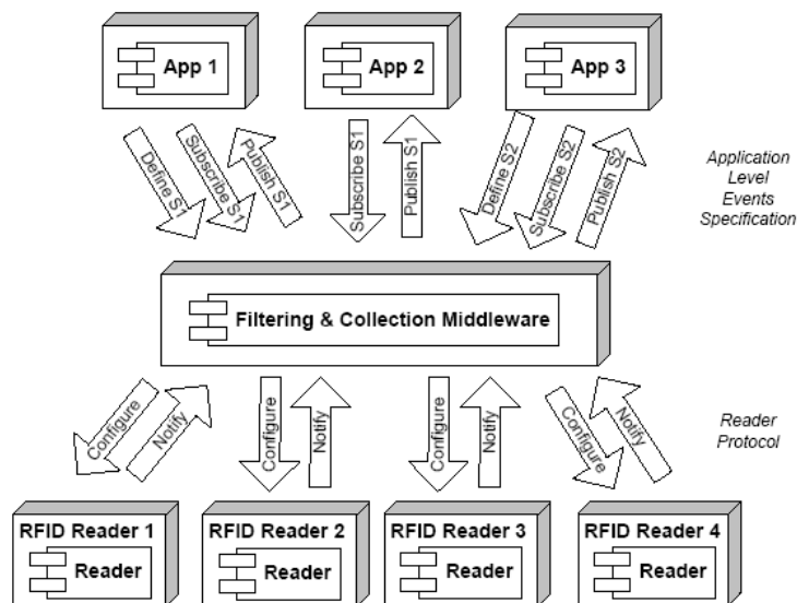
Figure 4. Filtering and collection middleware
