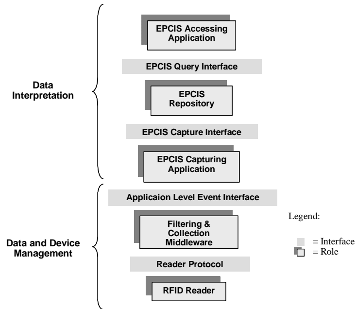
Figure 1. EPC Network Roles and Interfaces [2]
