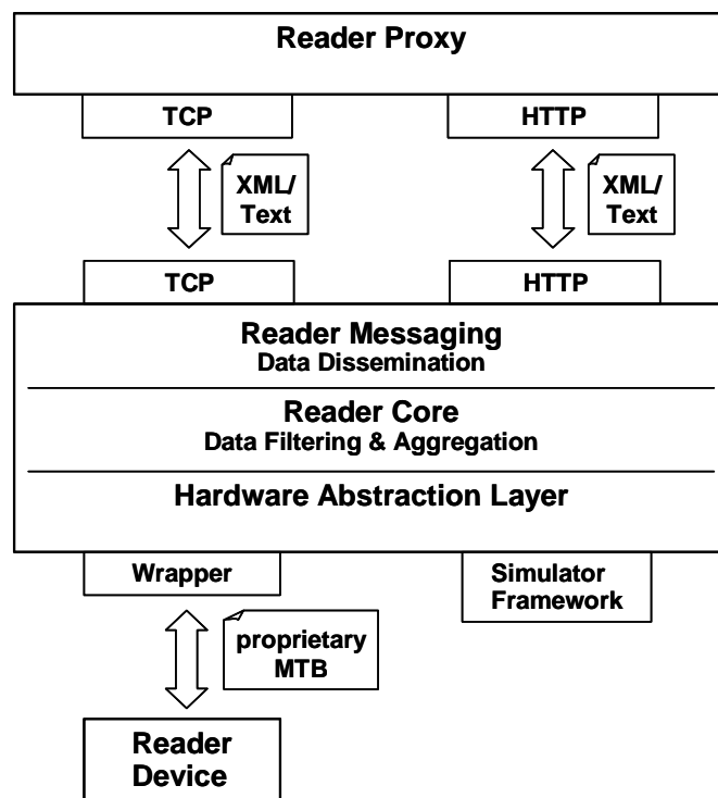
Figure 2. Accada Reader Implementation
