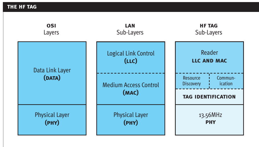
Figure 1: The HF TAG considers only protocols that operate in the Data Link and Physical Layers.
