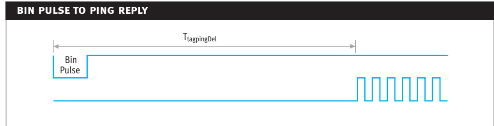
Figure 16: Bin Pulse to PingID Reply
