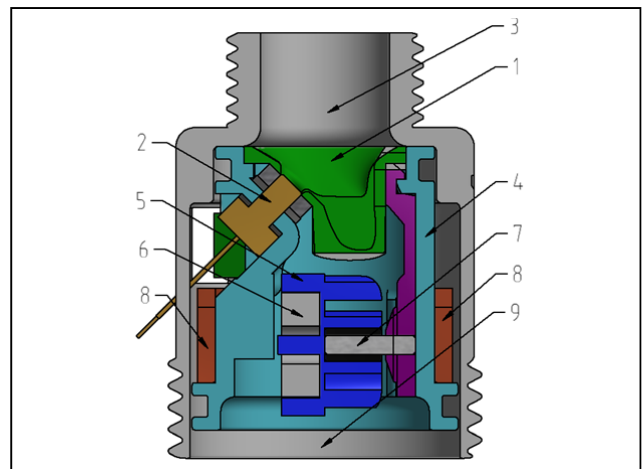
Figure 1: Cross section of the micro-generator unit: 1- turbine nozzle; 2 - thermistor; 3 - measurement unit water inlet; 4 - micro-generator tube; 5 - turbine wheel; 6 - generator magnet; 7 - generator wheel axle; 8 - generator coil; 9 - measurement unit water outlet
